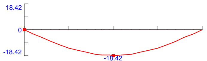
Deflection Diagram (Y) ( 1/100 in )
