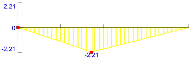
Moment Diagram (Y) (kip-ft)
